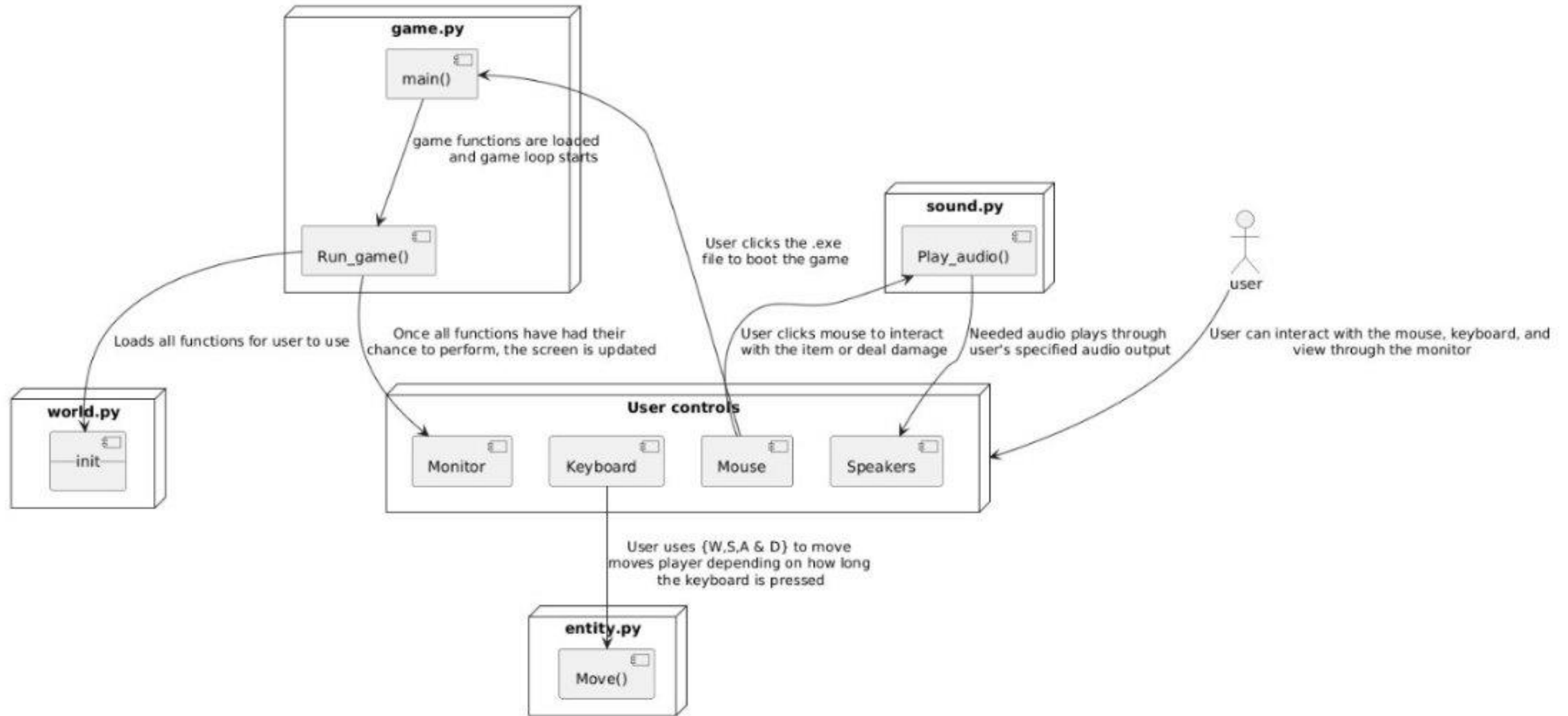
Game Deployment Diagram
